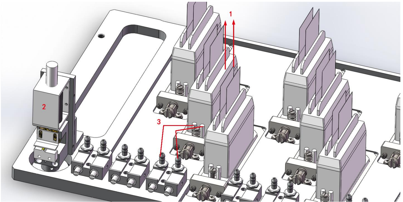
Installation Diagram of Print Head Ricoh G5
