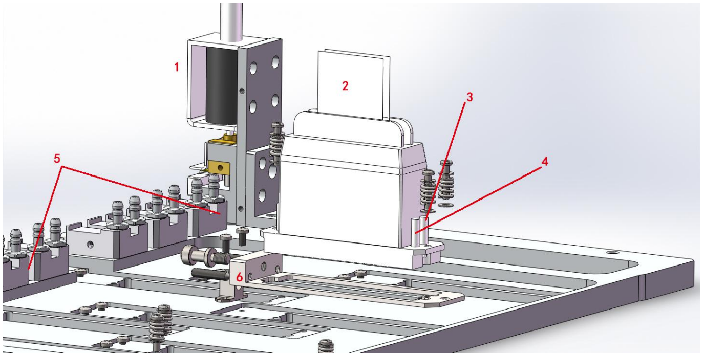
Installation Diagram b of Print Head Ricoh G5
