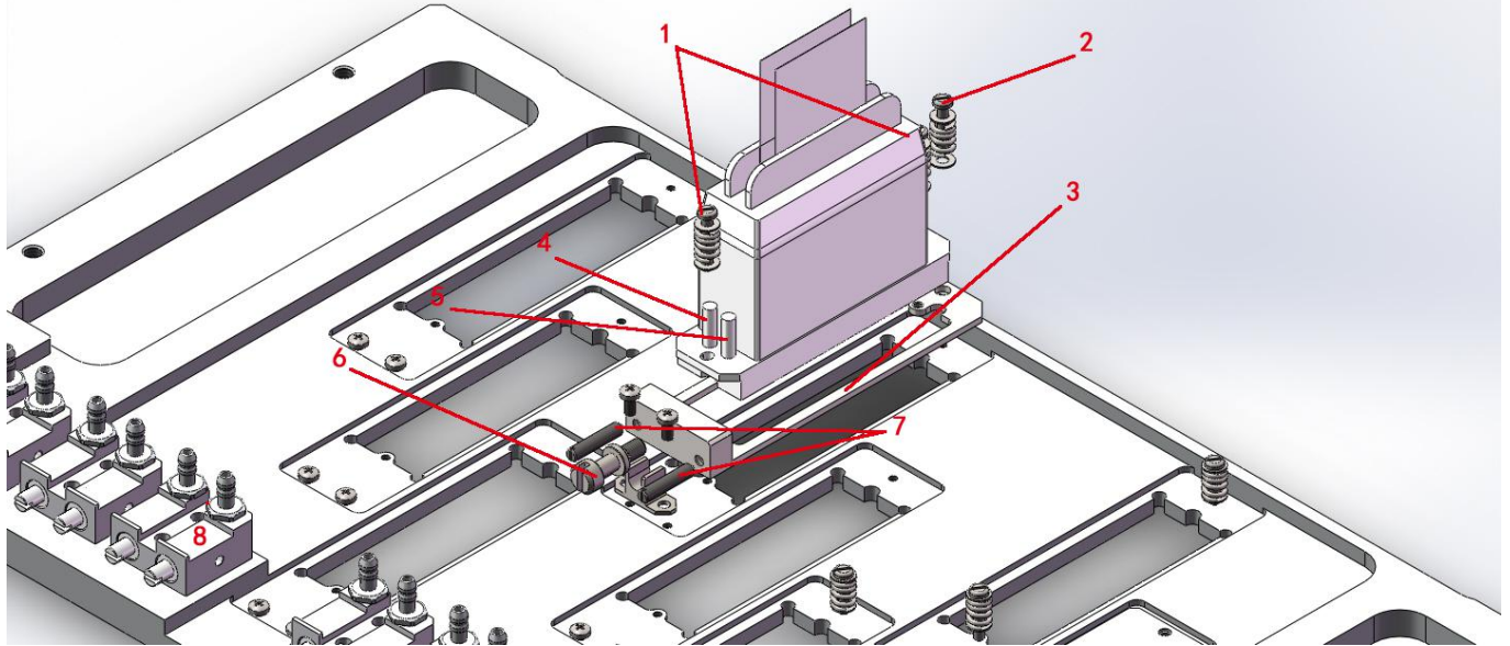
Installation Diagram a of Print Head Ricoh G5
